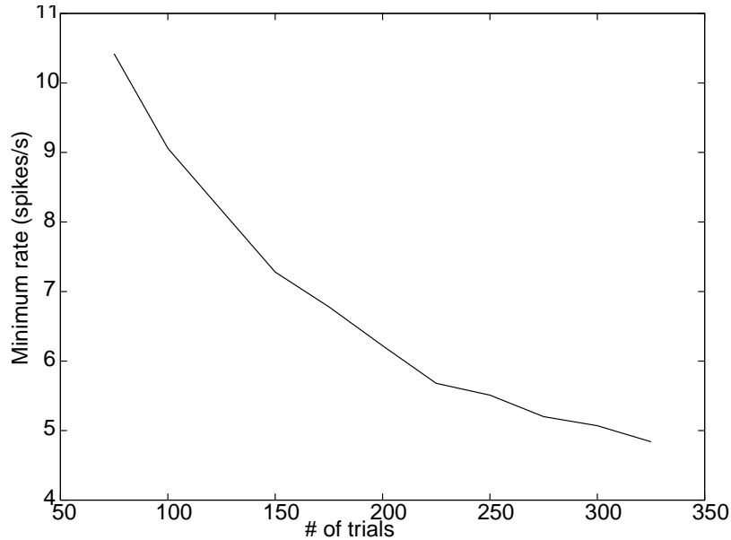
Figure 7: Minimum rates where mean UE frequency = 2\sigma .
